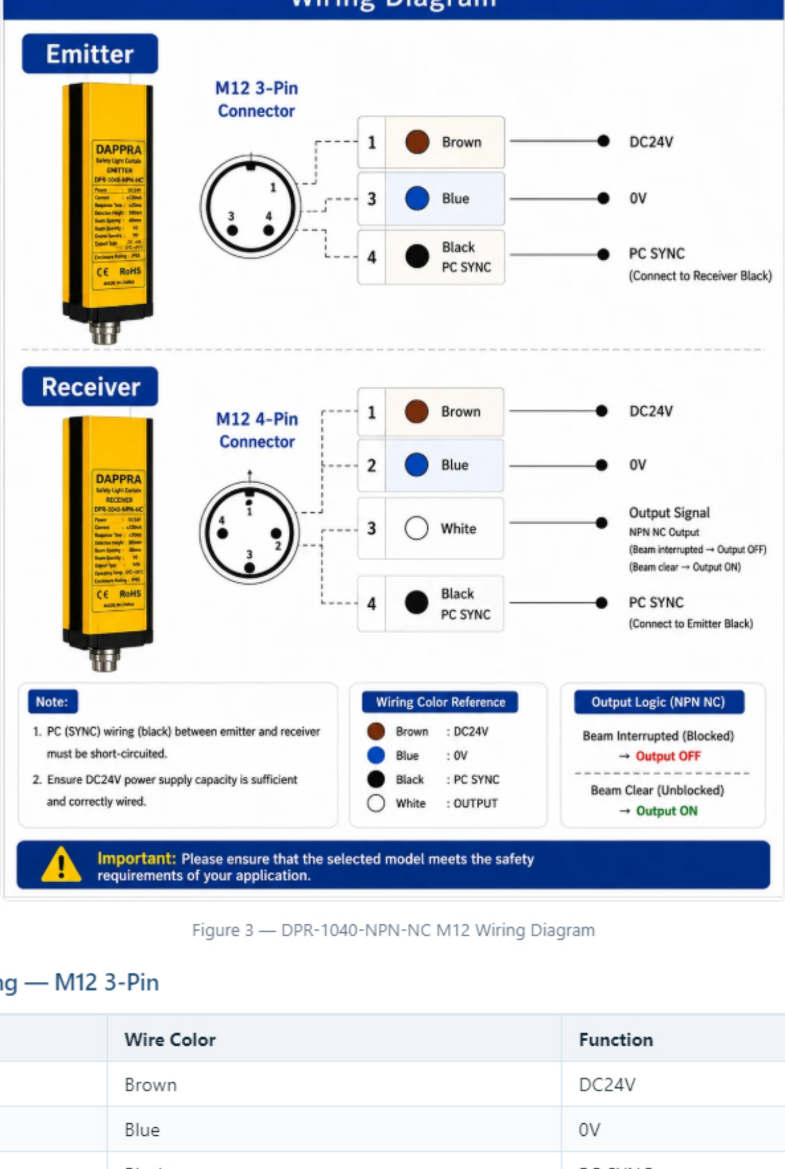
Figure 3 — DPR-1040-NPN-NC M12 Wiring Diagram
