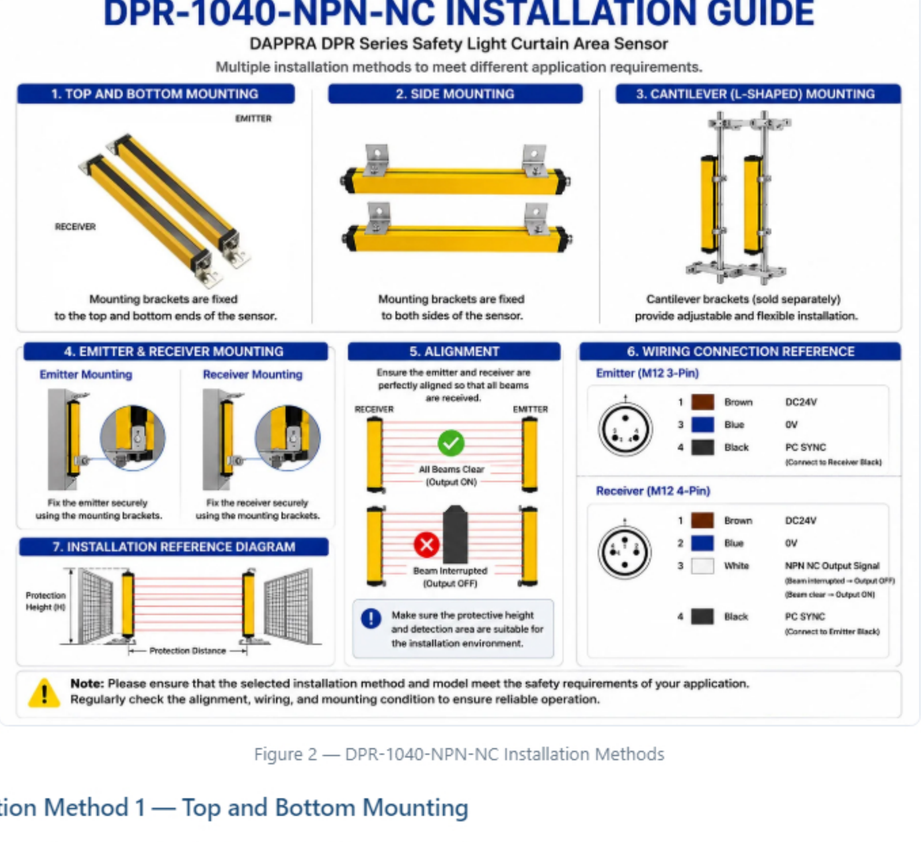
Figure 2 — DPR-1040-NPN-NC Installation Methods
