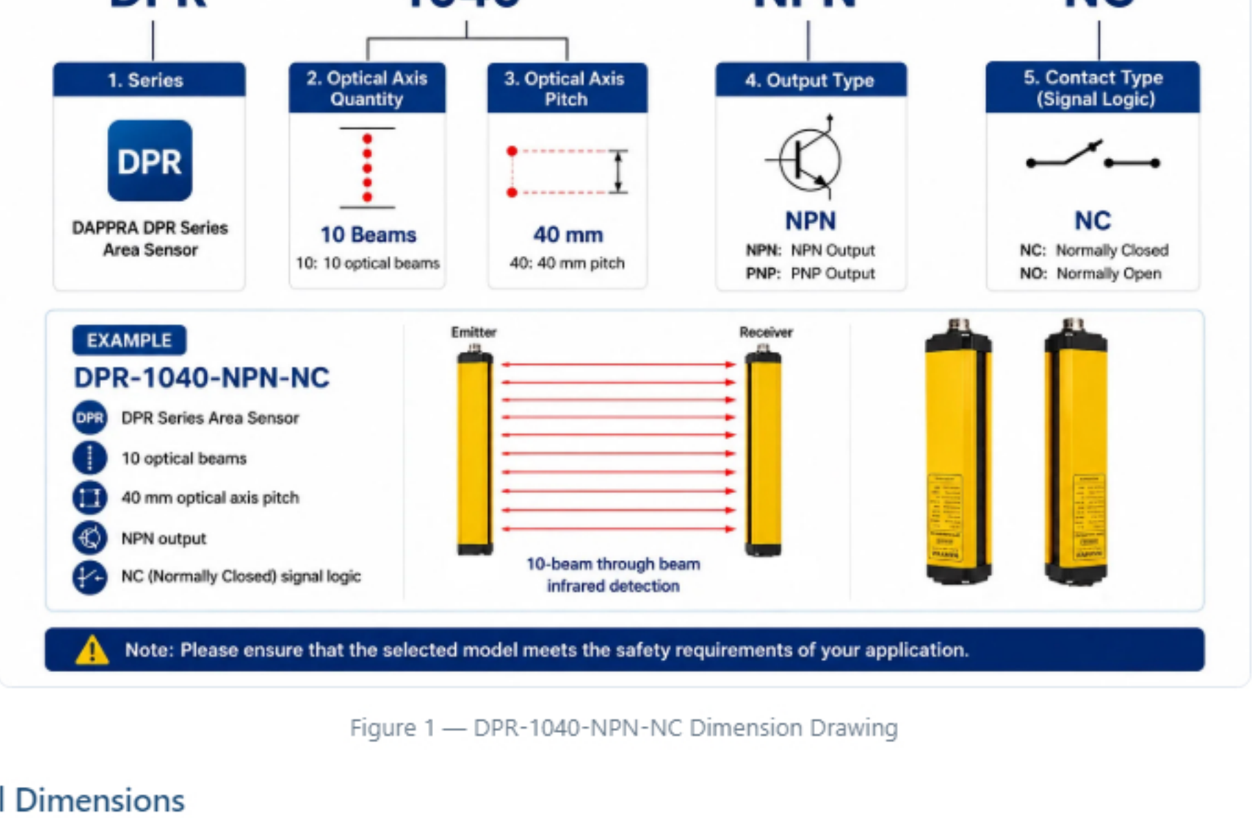
Figure 1 — DPR-1040-NPN-NC Dimension Drawing
